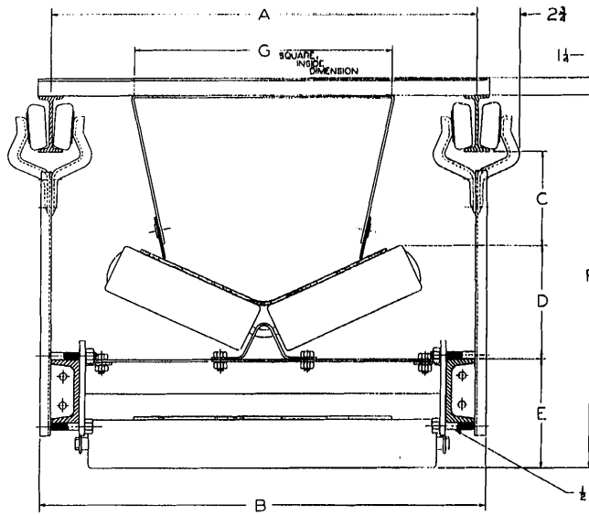
MODEL 3220 DUAL ROLL CONVEYOR CROSSSECTIONS - TROLLEY WHEEL ASSEMBLY
