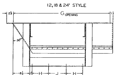
OPEN STYLE HOPPER DUAL ROLL CONVEYOR
