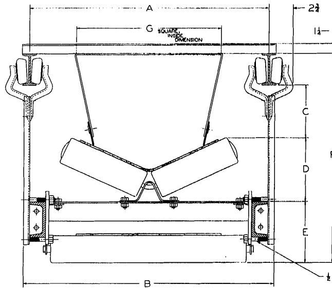
MODEL 3220 DUAL ROLL CONVEYOR CROSSECTIONS - TROLLEY WHEEL ASSEMBLY
