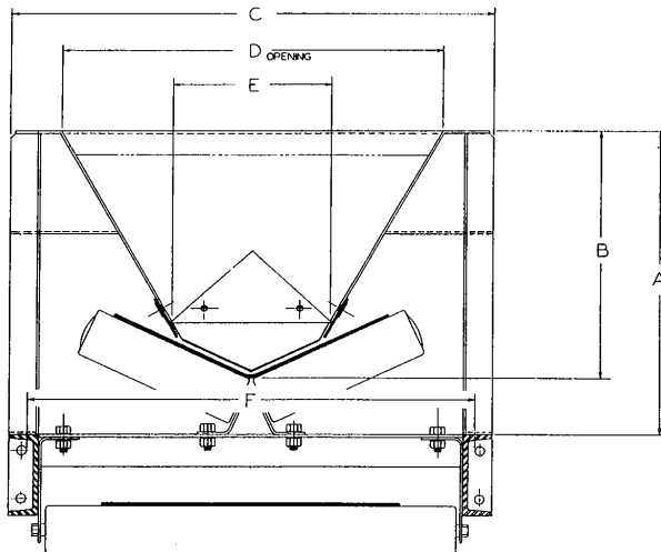
OPEN STYLE HOPPER DUAL ROLL CONVEYOR
