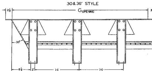
OPEN STYLE HOPPER DUAL ROLL CONVEYOR
