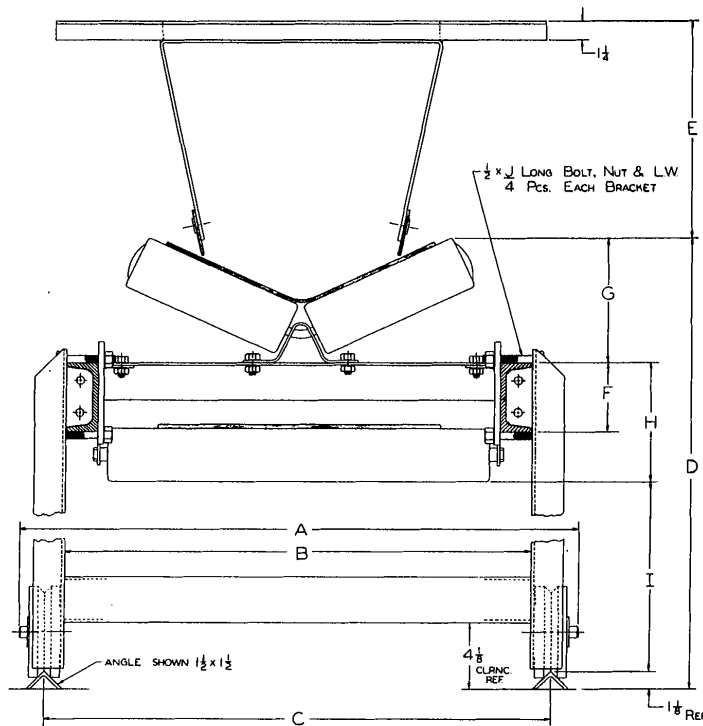
MODEL 3220 VEE TRACK WHEEL ASSEMBLY
