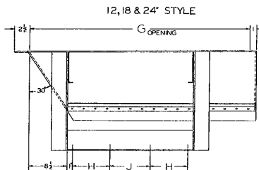
OPEN STYLE HOPPER DUAL ROLL CONVEYOR
