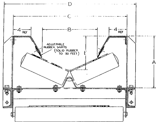
MODEL 3220 CROSSSECTION - CONTINUOUS SKIRTING DUAL ROLL CONVEYOR
